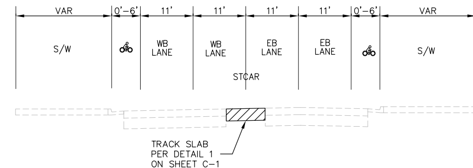
STA R 55+50 TO R 57+00 TOWER GATEWAY NTS
