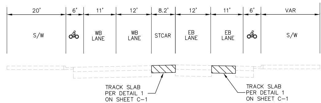
STA R 52+00 TO STA R 53+46 TOWER GATEWAY NTS
