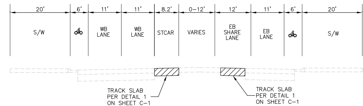
STA R 53+46 TO STA R 55+50 TOWER GATEWAY NTS
