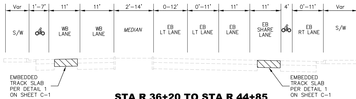
STA R 36+20 TO STA R 44+85 TOWER GATEWAY NTS
